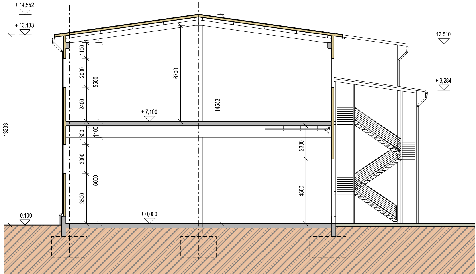
REZ A - A
